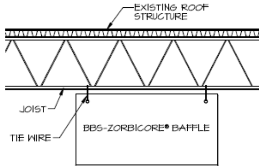
FRONT ELEVATION SCALE: 3/16"=1'-0"
