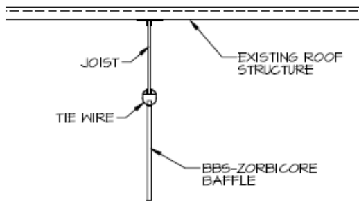
SIDE ELEVATION SCALE: 3/16"=1'-0"
